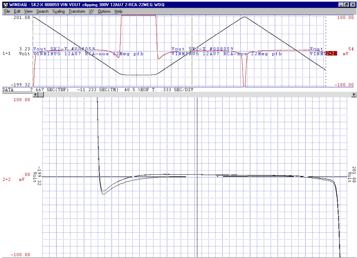
SK2-X VIN&VOUT vs Supplies 1 300V.gif
